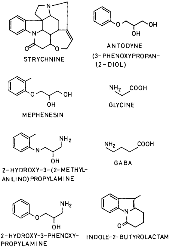
Figure 10 Structures of substances referred to in text
