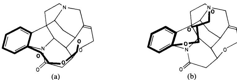
Figure 13 Two possible fits of the mephenesin molecule to that of strychnine. Structure (a) represents the lowest energy conformation.
