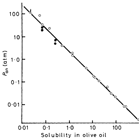
Figure 3 The correlation of anaesthetic pressures with solubility in olive oil. The anaesthetic potency of a substance is seen to be directly proportional to its solubility in this solvent. The filled circles represent fluorine compounds
