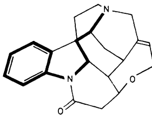
Figure 11 Structure of strychnine with that part of the molecule believed to confer convulsant activity emphasized
