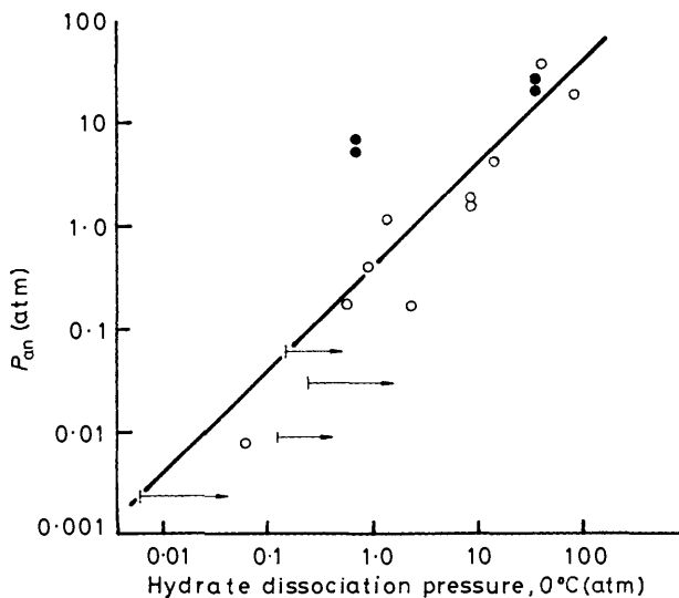
Figure 2 The correlation of anaesthetic pressures with hydrate dissociation pressures at 273K. The arrows indicate anaesthetic substances that do not form hydrates at their saturated vapour pressures. The filled circles represent fluorine compounds
