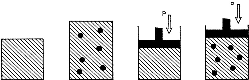
Figure 6 Diagrammatic representation of the constant volume hypothesis
